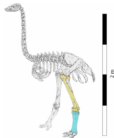
Fig. 2. A. maximus skeletal reconstruction. Highlighted elements correspond to Figs. 3 (blue) and 4 (yellow). Adapted from original drawing by A. Rasolo.
