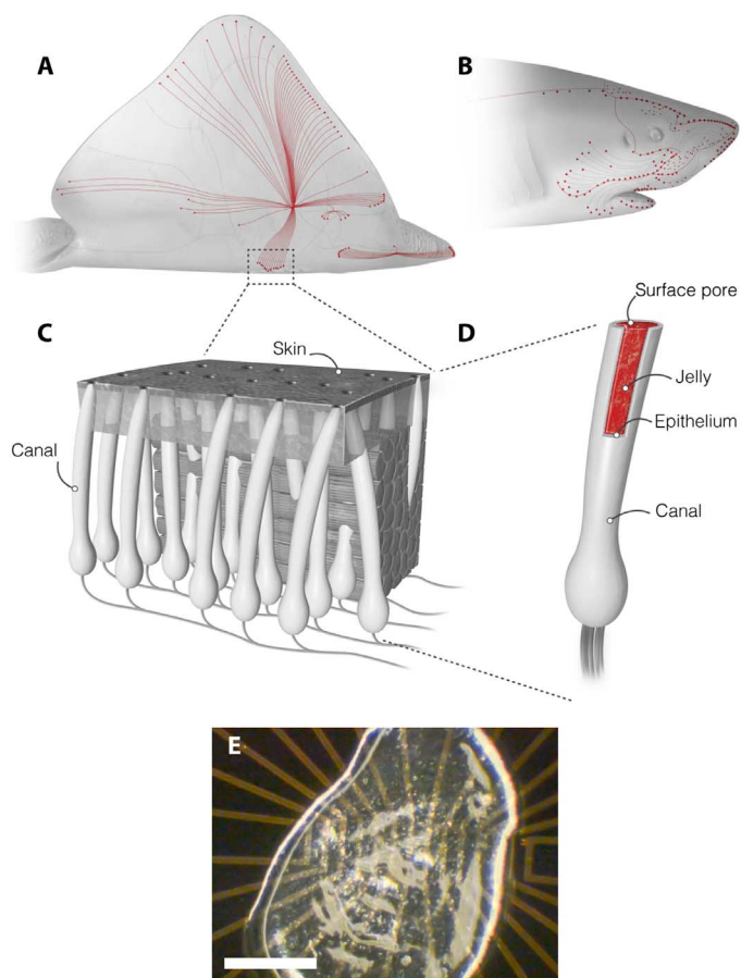
Fig. 1. The AoL. (A and B) Skates and sharks locate their prey by detecting the weak electric fields naturally generated by biomechanical activity. (C) A network of electroreceptive organs called the AoL is responsible for this sense. (D) An individual ampulla consists of a surface pore connected to a set of electroreceptive cells by a long jelly-filled canal. Sharks and skate can sense fields as small as 5 nV/cm despite canals traveling through up to 25 cm of noisy biological tissue. (E) A sample of the AoL jelly on an electrical device is presented. Scale bar, 0.5 mm.
