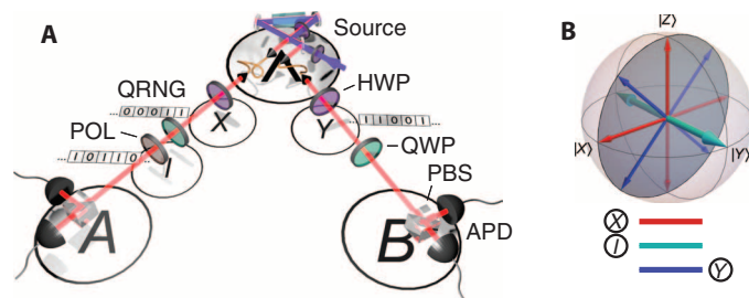
Fig. 2. The experimental setup. (A) Pairs of photons are generated via spontaneous parametric down-conversion in a periodically poled KTP crystal, using the Sagnac design of Fedrizzi et al. (48). The degree of polarization entanglement between the two photons can be continuously varied by changing the polarization angle \gamma of the pump laser. Alice and Bob perform measurements in the equatorial plane of the Bloch sphere using a half-wave plate (HWP) and a polarizing beam splitter (PBS). Additional quarter-wave plates (QWPs) can be used for quantum state tomography of the initial entangled state. In the interventionist experiment, an additional combination of QWP and polarizer (POL) is used between Alice's basis choice and her measurement. Causal variables are indicated using the notation of Fig. 1A. Note that \Lambda can represent an arbitrary hidden variable acting as a common cause for the observed outcomes, which need not necessarily originate at the source. (B) Alice's (red) and Bob's (blue) measurement bases and the intervention direction (cyan) on the Bloch sphere. QRNG, quantum random number generator; APD, avalanche photodiode.
