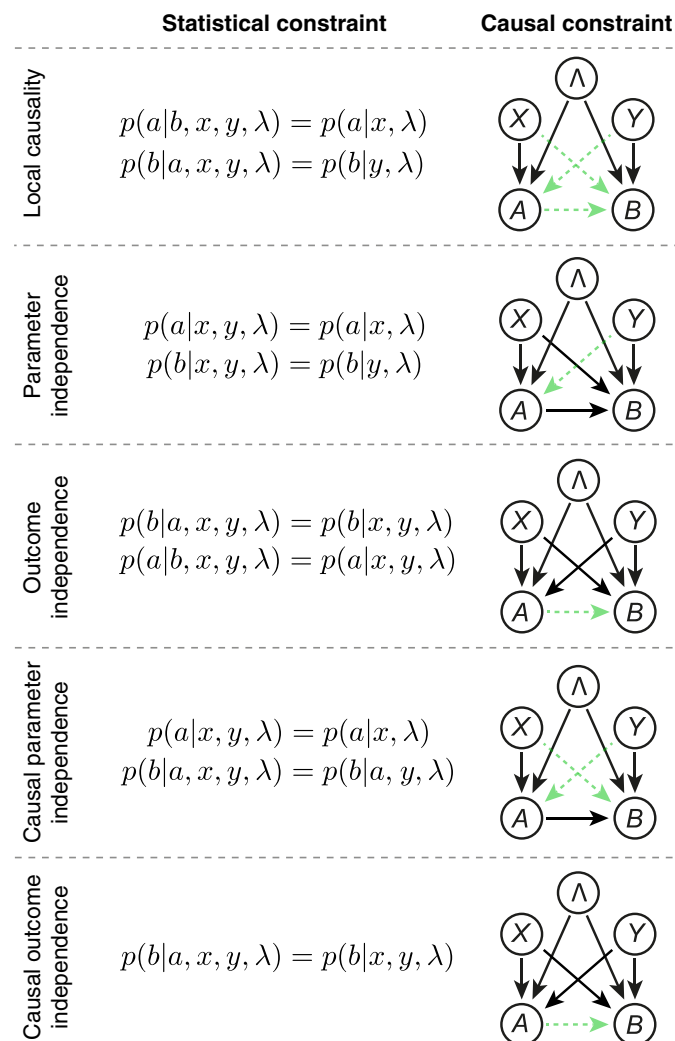
Fig. 5. Comparison of various constraints on the causal structure of Bell’s theorem. The causal links forbidden by the respective assumption are shown in dashed green lines. Note that the statistical constraints implied by causal parameter independence are asymmetric in a and b , and swapping them would result in a causal structure where the arrow between A and B is reversed. Our experimental test applies to both of these structures and any convex combination of them.
