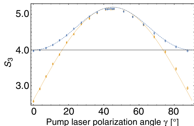
Fig. 4. Observed values S_3 for a variety of quantum states of the form \cos\gamma|HV\rangle + \sin\gamma|VH\rangle . The orange data points are observed using a fixed measurement scheme (optimal for the maximally entangled state \gamma = 45^\circ ), with the dotted, orange line representing the corresponding theory prediction. The blue data points and blue dashed theory line correspond to the case where measurement settings were optimized for the prepared states (see the Supplementary Materials for details). The black line represents the bound of inequality (5); any point above this line cannot be explained causally by a model of the form in Fig. 1B. Error bars correspond to 3\sigma statistical confidence intervals.
