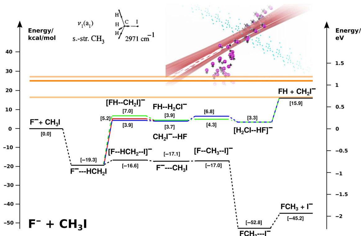
Fig. 1. Stationary points along the reaction coordinate of the reaction \text{F}^- + \text{CH}_3\text{I} for the \text{S}_{\text{N}}2 and the proton transfer reaction channel [taken from (33)]. Both reaction channels proceed via the same pre-reaction complex, in which the fluoride anion is hydrogen-bonded to an H atom. The transition state of the \text{S}_{\text{N}}2 is submerged, whereas a barrier exists for the proton transfer. Intrinsic reaction coordinate computations find three interconnected proton transfer pathways. The [\text{FH}\cdots\text{CH}_2\text{I}]^- transition state of the most direct pathway, which is marked in green, is used for the SVP analysis. The relative translational collision energies are marked with the light orange lines, and the total translational and vibrational energy of the CH-stretch excited reactants is marked with the bright orange line. The inset shows a sketch of the scattering experiment with \text{CH}_3\text{I} excited in the symmetric ( a_1 ) CH stretching mode at 2971 \text{ cm}^{-1} or 0.37 eV.
