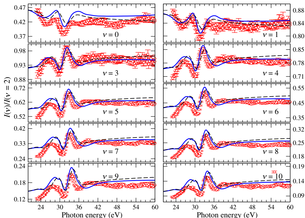
Fig. 1. Vibrationally resolved photoionization cross sections normalized to that for the v=2 state of \text{H}_2^+ as a function of photon energy. Circles with error bars: Experimental data. Full lines: Ab initio calculation. Dashed lines: Fit to the experimental data by using the extended Fano model described in the text [see also (35)].
