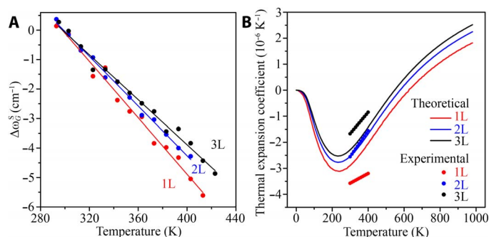
Fig. 6. TECs of 1-3L BN. (A) The G band frequency shifts as a function of temperature and the corresponding fittings of 1-3L BN bound to SiO 2 /Si using TECs as fitting parameters. (B) Experimental (dots) and theoretical (lines) curves of the TECs of the 1-3L BN.
