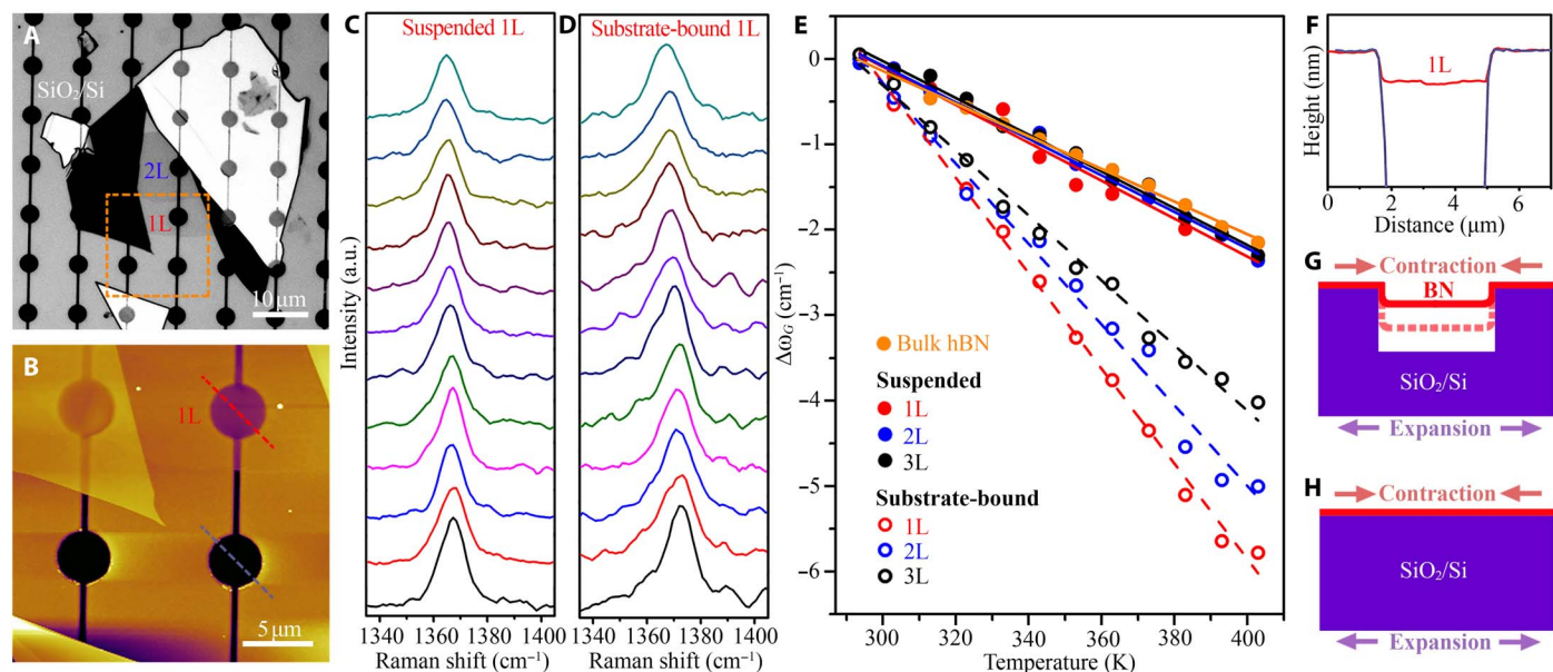
Fig. 1. The first-order temperature coefficients. (A) Optical image of a 1-2L BN on SiO 2 /Si substrate with prefabricated microwells. (B) AFM image of the squared area in (A). (C and D) Raman G bands of the 1L BN suspended over and bound to SiO 2 /Si at different heating stage temperatures from 293 to 403 K with an interval of 10 K. a.u., arbitrary units. (E) Summarized G band frequency changes of the suspended and substrate-bound 1-3L BN as a function of temperature and the corresponding linear fittings. (F) AFM height traces of the dash lines in (B). (G and H) Schematic diagrams of the thermal expansion of suspended and substrate-bound BN nanosheets.
