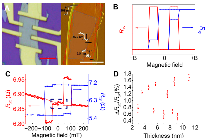
Fig. 1. Overview of the MR effect in FGT/graphite/FGT heterostructures. (A) Optical and AFM images of an FGT/graphite/FGT heterostructure. The device number is FPC3. Scale bars, 5 \mu m. The regions surrounded by the blue line, red line, and yellow line represent the top FGT layer, graphite layer, and bottom FGT layer, respectively. (B) Schematic diagram for the transport behavior of a typical GMR effect. (C) Field-dependent R_{xx} and R_{xy} measurements of an FGT/graphite/FGT heterostructure (sample FPC3) at 50 K. A loop surrounded by a dark blue dashed line is shown in the R_{xx}(B) curve. (D) \Delta R_{xx}/R_{xx} values for samples with various thicknesses of graphite layer. All the data are calculated for measurements at 50 K. The error bars come from the noise of the measurement.
