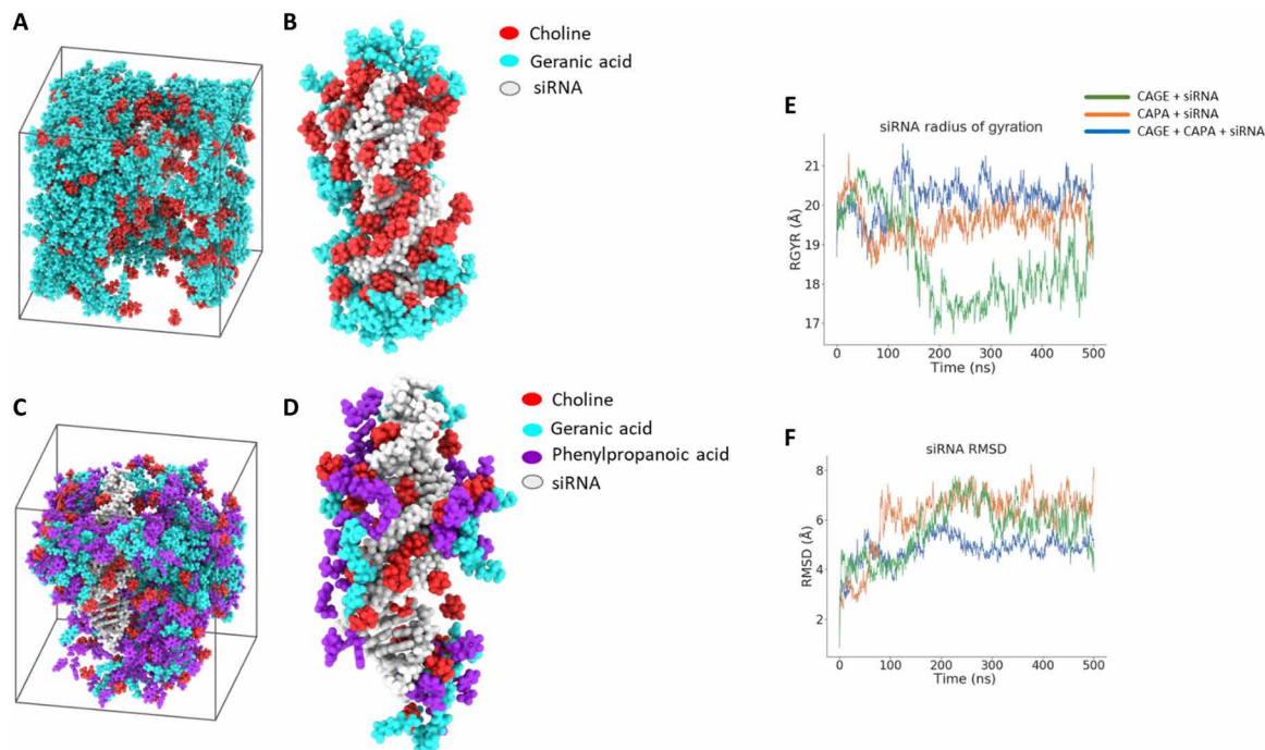
Fig. 2. MD simulation identifies the extent of IL-siRNA interaction for enhanced solvation and stability. (A and B) Snapshot of simulation unit cell for CAGE and siRNA (A) and CAGE components found within 10 Å of siRNA (B) under periodic boundary conditions for 500 ns. (C and D) Snapshot of simulation unit cell for the optimized IL combination (CAGE and CAPA, 1:1) and siRNA (C) and IL species found within 10 Å of siRNA (D) under similar conditions. (E and F) Radius of gyration (RGYR) (E) and root mean square deviation (RMSD) (F) obtained over the course of 500 ns for CAPA and the IL combination (CAGE and CAPA) in contrast to CAGE (control).
