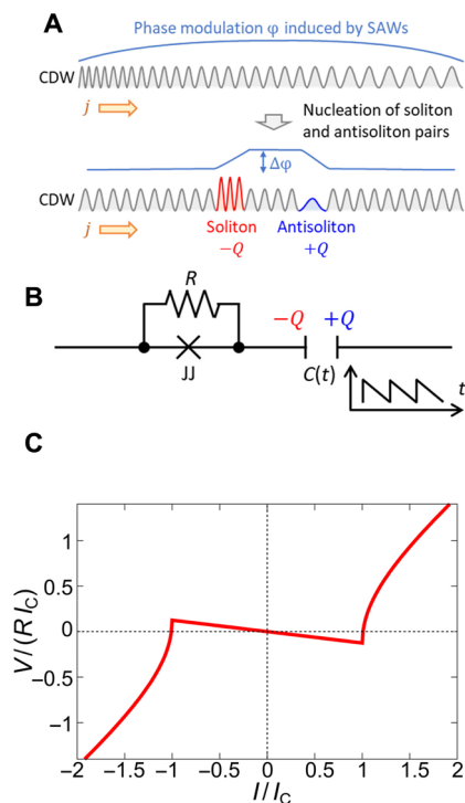
Fig. 4. Theoretical model to reproduce the negative resistance. (A) Schematics of nucleation of soliton and antisoliton pairs. When the SAW is irradiated to the CDW state, the CDW phase \phi is modulated over the wavelength of the SAW. Instead of modulating the CDW over the wavelength, it is more stable to nucleate soliton and antisoliton pairs in the CDW state. In the superconducting state, local charges ( -Q , +Q ) are accumulated, resulting in a temporal and local capacitance C(t) and a phase difference \Delta\phi of 2\pi . (B) Circuit model used in the calculation (see the Supplementary Materials for more details). We assume a resistively shunted Josephson junction (JJ), which is capacitively coupled via C(t) . The change in C(t) is synchronized with the frequency of the SAW. We assume a sawtooth wave function for C(t) . (C) Typical I - V curve calculated with the above capacitively coupled Josephson junction model. The horizontal and vertical axes are normalized by I_C and the product of the resistance R of the normal state and I_C , respectively.
