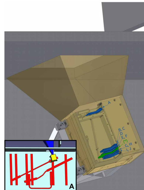
Fig. 2. Schematic view of the LND sensor head and its accommodation in the Chang'E 4 payload compartment. The LND detector system consists of 10 dual-segment silicon SSDs (A to J) shown and labeled in blue. They are arranged such as to form a particle telescope that views the sky through an opening of the payload compartment. The structure shown in green absorbs thermal neutrons and is irrelevant for this paper. This opening in the payload compartment (indicated by gray walls) is closed during the lunar night and reopened in the lunar morning. Multilayer insulation is shown in gold and insulates the LND sensor head, which is mounted to the side panel of the payload compartment with an Al bracket also shown in gray. Inset A shows LND's location on the payload panel (in pale blue) together with its \text{NH}_3 thermal control system (TCS) indicated in red.
