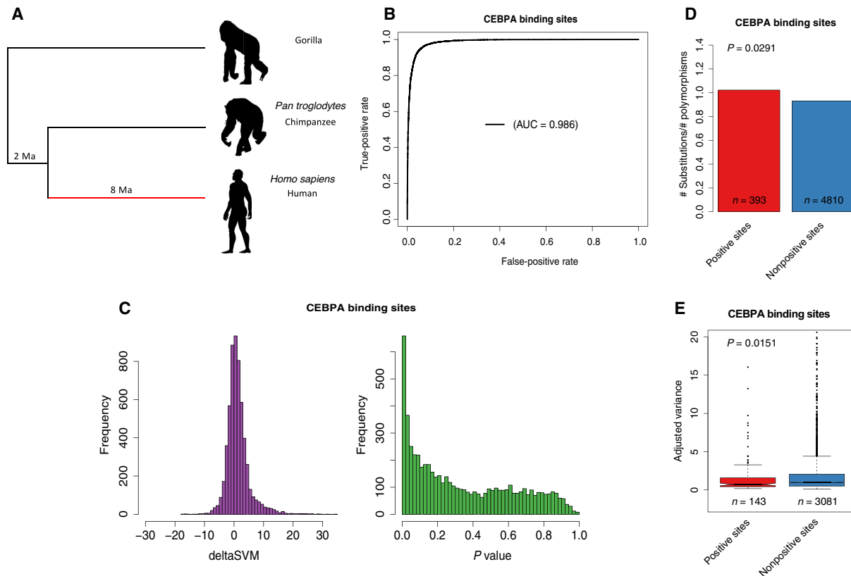
Fig. 3. Human CEBPA binding site study. (A) Topological illustration of the phylogenetic relationships between human, chimpanzee, and gorilla. We detected positive selection that occurred on the lineage of human after divergence from chimpanzee, as indicated by the red branch. (B) ROC curve for gkm-SVM classification performance on CEBPA binding sites (fivefold cross-validation). The AUC value represents the area under the ROC curve and provides an overall measure of predictive power. (C) The left graph is the distribution of deltaSVM. The right graph is the distribution of deltaSVM P values (test for positive selection). (D) Ratio between the number of substitutions and the number of polymorphisms [single-nucleotide polymorphisms (SNPs)] for CEBPA binding sites. Positive sites are binding sites with evidence of positive selection (deltaSVM P value < 0.01 ). The P value from Fisher's exact test is reported above the bars. (E) Comparison of expression variance (adjusted variance) of putative target genes (closest gene to a TFBS) between positive sites and nonpositive sites. The number of binding sites in each category is indicated below each box. The P values from a Wilcoxon test comparing categories are reported above boxes. Positive sites are binding sites with evidence of positive selection (deltaSVM P value < 0.01 ).
