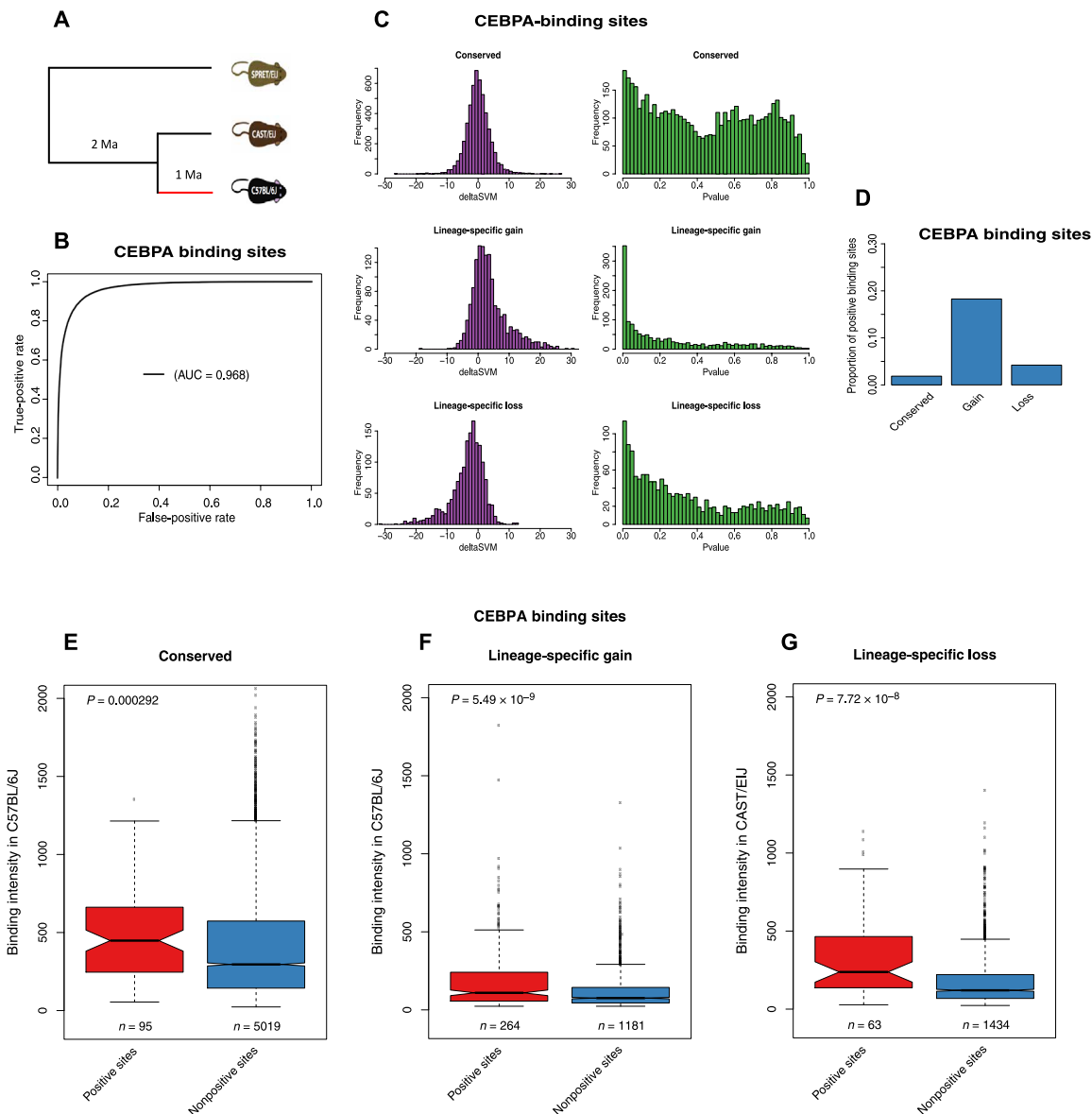
Fig. 2. Mouse CEBPA binding sites study. (A) Topological illustration of the phylogenetic relationships between the three mouse species used to detect positive selection on CEBPA binding sites. We want to detect positive selection that occurred on the lineage of C57BL/6J after divergence from CAST/EJ, as indicated by the red branch. Ma, million years. (B) Receiver operating characteristic (ROC) curve for gkm-SVM classification performance on CEBPA binding sites (fivefold cross-validation). The AUC value represents the area under the ROC curve and provides an overall measure of predictive power. (C) The left-hand graphs are the distributions of deltaSVM. The right-hand graphs are the distributions of deltaSVM P values (test for positive selection). (D) Proportion of CEBPA binding sites with evidence of positive selection. (E to G) The number of binding sites in each category is indicated below each box. The P values from a Wilcoxon test comparing categories are reported above boxes. Positive sites are binding sites with evidence of positive selection (deltaSVM P value < 0.01 ). (E) Conserved binding sites. (F) Lineage-specific gain binding sites. (G) Lineage-specific loss binding sites. We compare the binding intensity from CAST/EJ, as an approximation for ancestral binding intensity, between positive loss binding sites and nonpositive loss binding sites.
