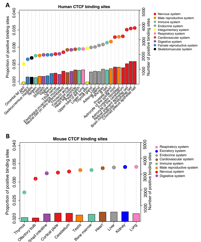
Fig. 4. Proportion of positive CTCF binding sites in different tissues or cell types. PBSs are binding sites with evidence of positive selection ( \Delta SVM P value < 0.01 ). Colors correspond to broad anatomical systems. (A) CTCF binding sites in 29 human tissues or cell types. (B) CTCF binding sites in 11 mouse tissues.
