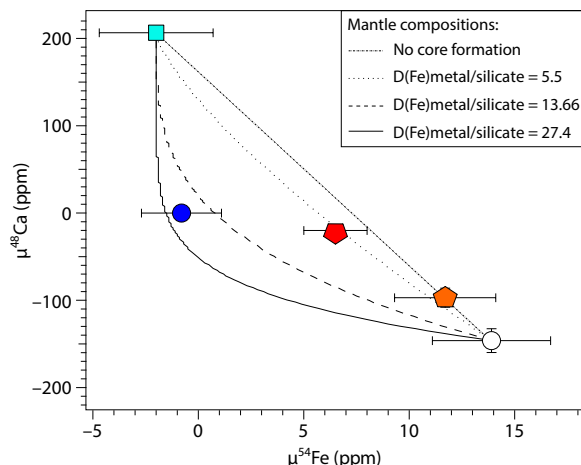
Fig. 3. Plot of \mu^{48}\text{Ca} versus \mu^{54}\text{Fe} of silicate mantles of inner solar system asteroids and planets and CI chondrites with possible accretion trajectories. \mu^{54}\text{Fe} values are shown versus \mu^{48}\text{Ca} data (10, 18) for the mantles of Earth, Mars, Vesta, and the UPB, where an increase in \mu^{48}\text{Ca} represents addition of CI-like solids to the planetary objects (18). Symbols and uncertainties are the same as in Fig. 2. Shown trajectories for the evolution of the \mu^{48}\text{Ca} - \mu^{54}\text{Fe} mantle composition of a growing planetary body in the inner solar system assume either no core formation or core formation on a planetary body with initially UPB-like composition and subsequent addition of CI-like dust with distinct degrees of iron partitioning between core and mantle [ D(\text{Fe})_{\text{metal/silicate}} ] that are held constant throughout accretion. We show the isotopic evolution of a putative mantle composition in \mu^{48}\text{Ca} - \mu^{54}\text{Fe} space for three D(\text{Fe})_{\text{metal/silicate}} values: one reflecting iron partitioning similar to that recorded by Earth today [ D(\text{Fe})_{\text{metal/silicate}} = 13.66 ], as well as for accretion under more reducing [ D(\text{Fe})_{\text{metal/silicate}} = 27.4 ] or under more oxidizing [ D(\text{Fe})_{\text{metal/silicate}} = 5.5 ] conditions. For simplicity, partitioning values are calculated by partitioning of only iron and nickel [ D(\text{Ni})_{\text{metal/silicate}} = 26.5 ] into the core.
