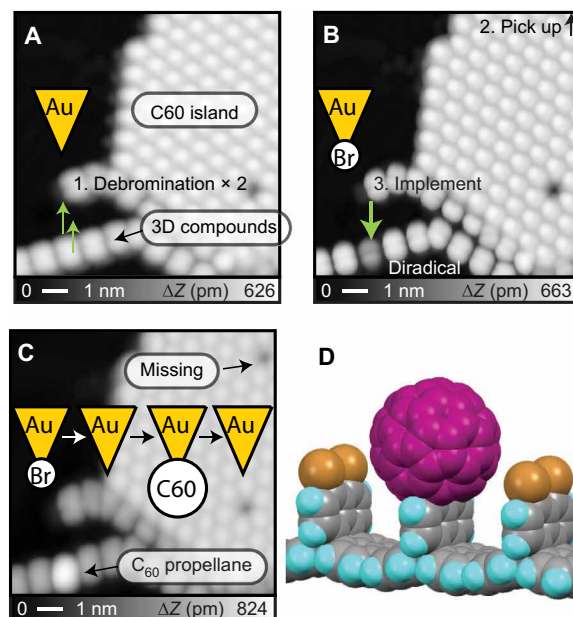
Fig. 3. Synthesis of C 60 -propellane complex. (A) STM topography of a C 60 island and 3D-OMC, taken with a Au tip. Green arrows indicate sites of the debromination. (B) STM topography after twice of the debromination, taken with a Br tip. A black arrow indicates the C 60 to be picked up from the island. A green arrow indicates the site to implement the C 60 from the tip. (C) STM topography after the synthesis of C 60 -propellane complex, taken with a Au tip. Insets show the schematic drawings of the tip apex. (D) Schematic drawing of C 60 -propellane complex. Measurement parameters: V = 200 mV and I = 2 pA in (A) and (B), and V = 1500 mV and I = 2 pA in (C).
