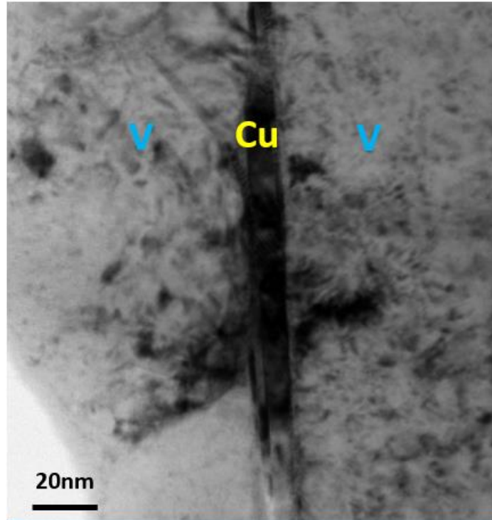
fig. S1. Cross-sectional TEM image of as-prepared V/Cu/V sample.
